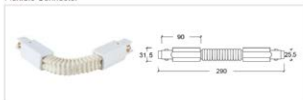
Flexible Connector
